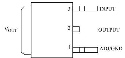
D Package (TO-252)
