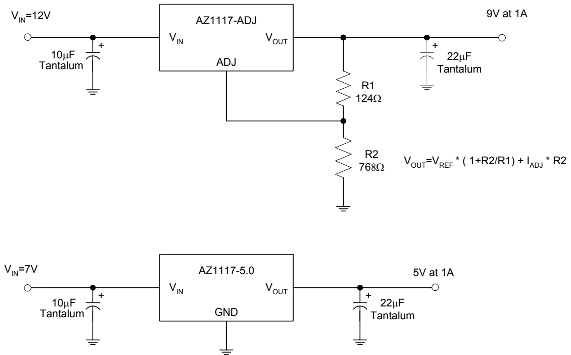
Figure 15. Typical Applications of AZ1117
