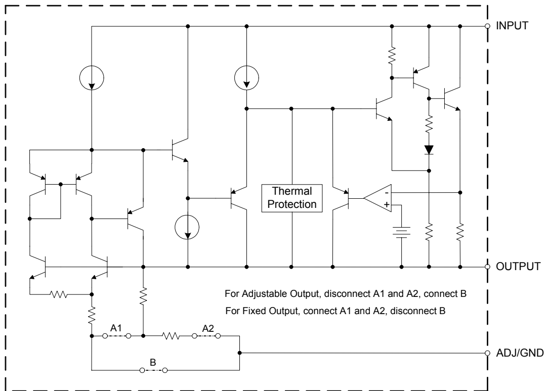
Figure 3. Functional Block Diagram of AZ1117
